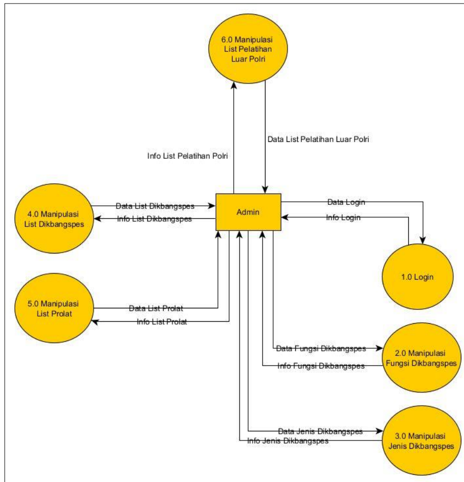
Gambar 5. DFD level 1
