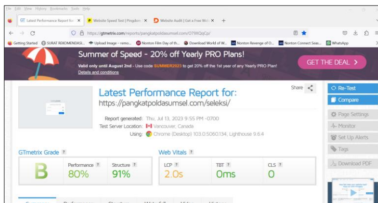
Gambar 15. Testing gtmatrix.com
