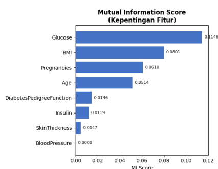
Gambar.2 Distribusi skor mutual information
